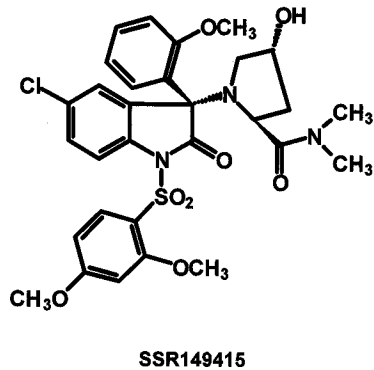
Fig. 1. Chemical structures of SSR149415 ((2 S , 4 R )-1-[5-chloro-1-[(2,4-dimethoxyphenyl)sulfonyl]-3-(2-methoxyphenyl)-2-oxo-2,3-dihydro-1 H -indol-3-yl]-4-hydroxy- N,N -dimethyl-2-pyrrolidine carboxamide, isomer(-)).
